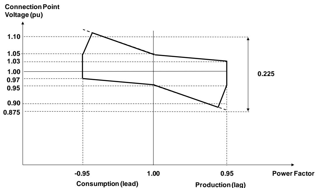
Figure 13.12 Reactive Power capability requirements (Power Park Modules operating at Registered Capacity, voltage above 33 kV)
