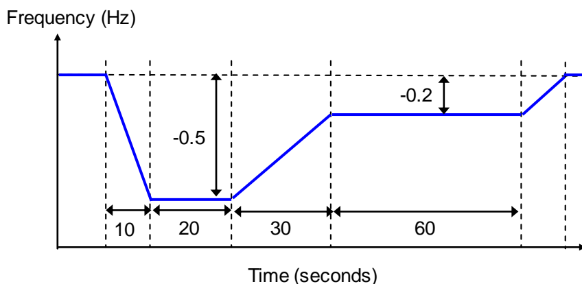
Figure C.7.4 Controller simulation
