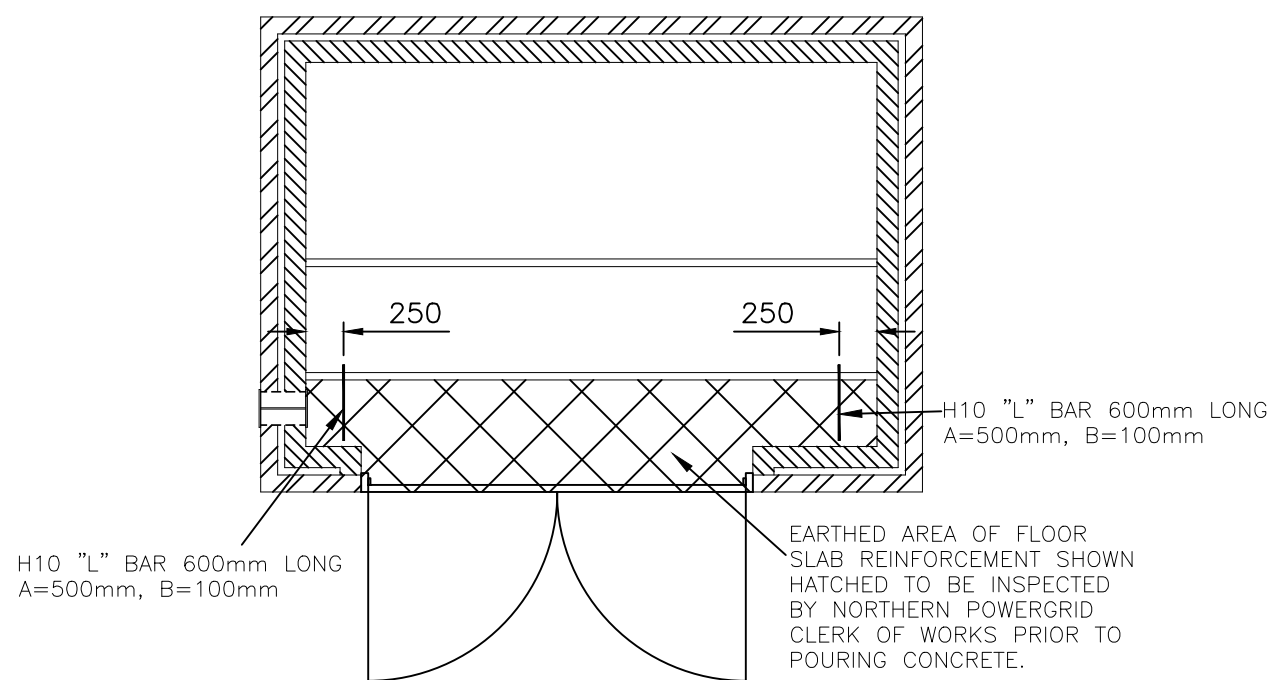
TYPICAL EXAMPLE SHOWING EARTH BAR POSITIONS
