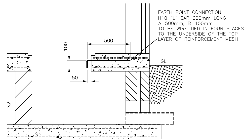
TYPICAL EXAMPLE OF A SECTION SHOWING EARTH BAR
